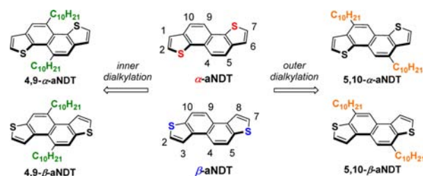
Figure 1. Molecular structures of \alpha -aNDT, \beta -aNDT, and four isomeric dialkylated aNDTs.
